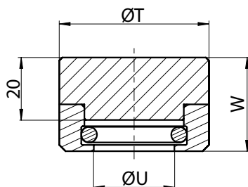
Pressure piece, complete - XKM 123 ... XKM 125
